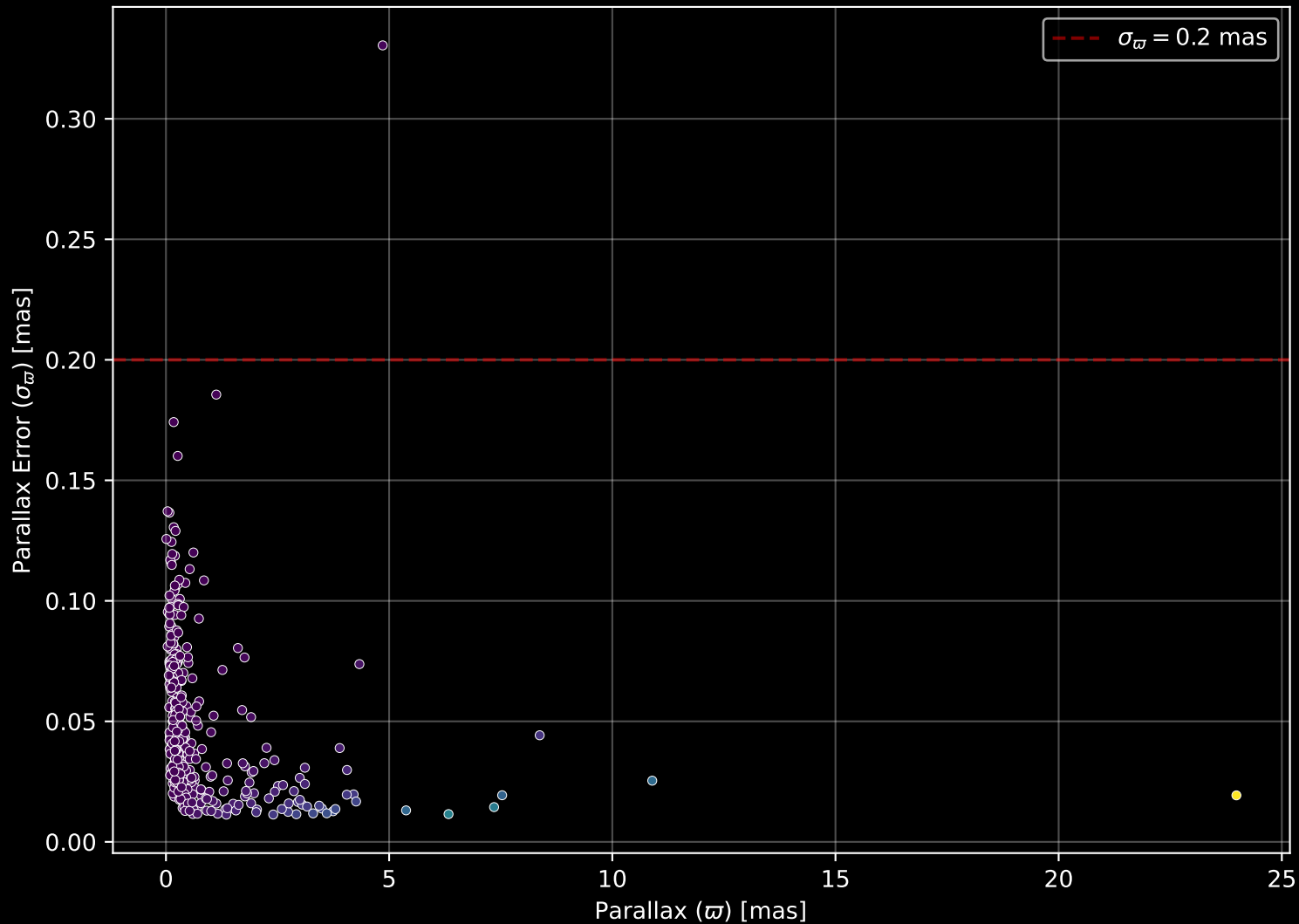
APOGEE DR17 Field: [120+04] Parallax Quality (n= 431)
