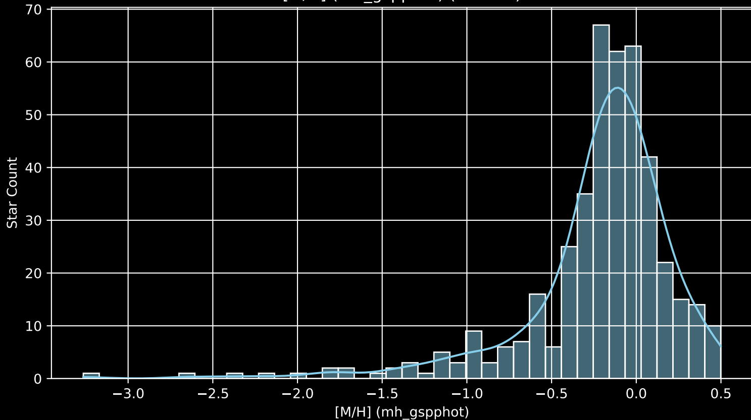
APOGEE DR17 Field: [120+04 [M/H] (mh_gspphot) (n= 426)
