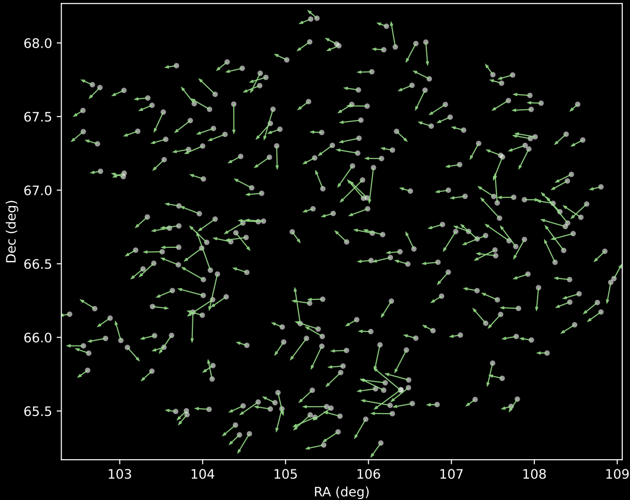
APOGEE DR17 Cluster 5 Proper Motion Vectors (n=265)
