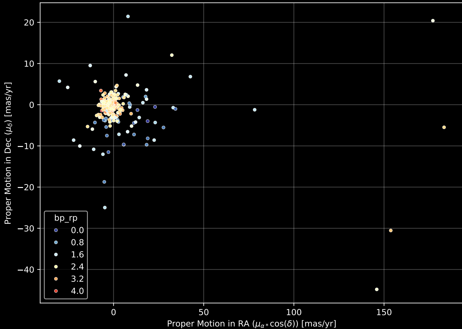
APOGEE DR17 Field: [120+04] Proper Motion Diagram (n= 431)
