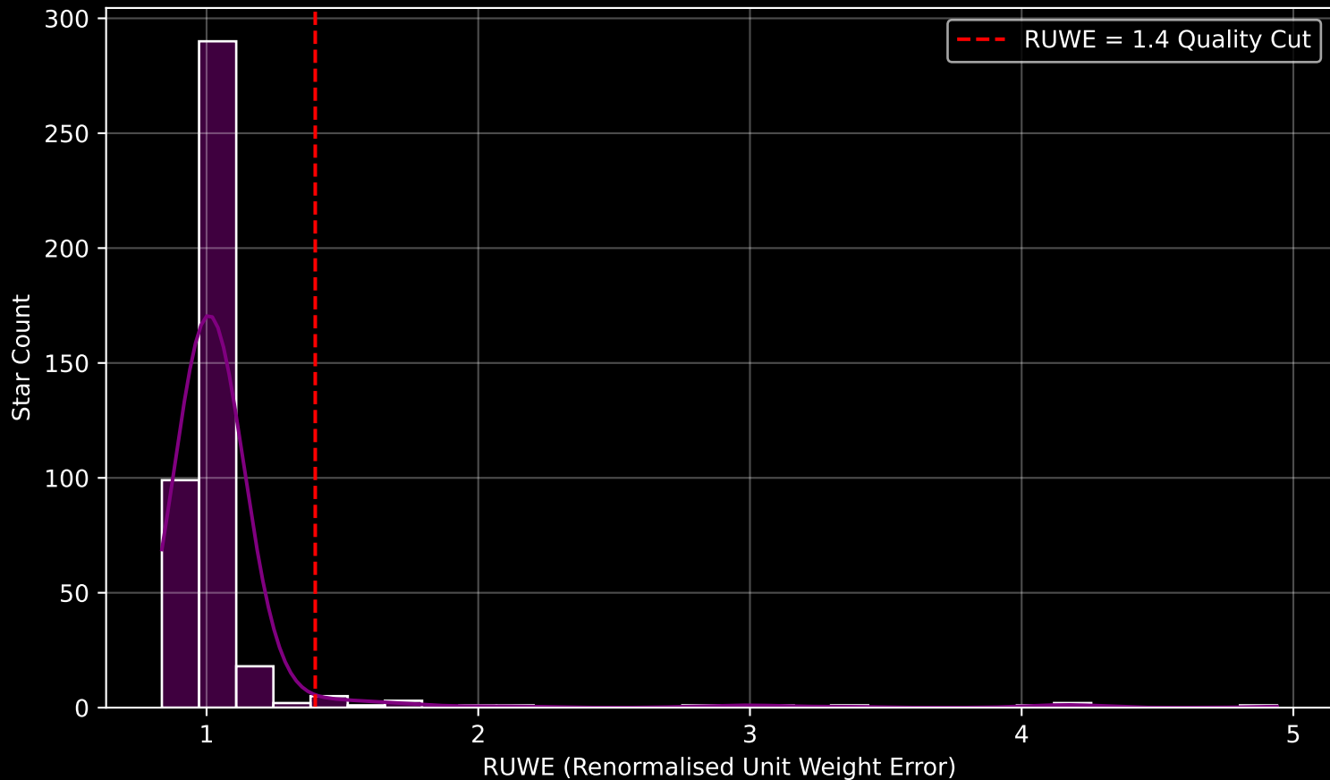
GAPOGEE DR17 Field [120+04] RUWE Distribution (n= 428)
